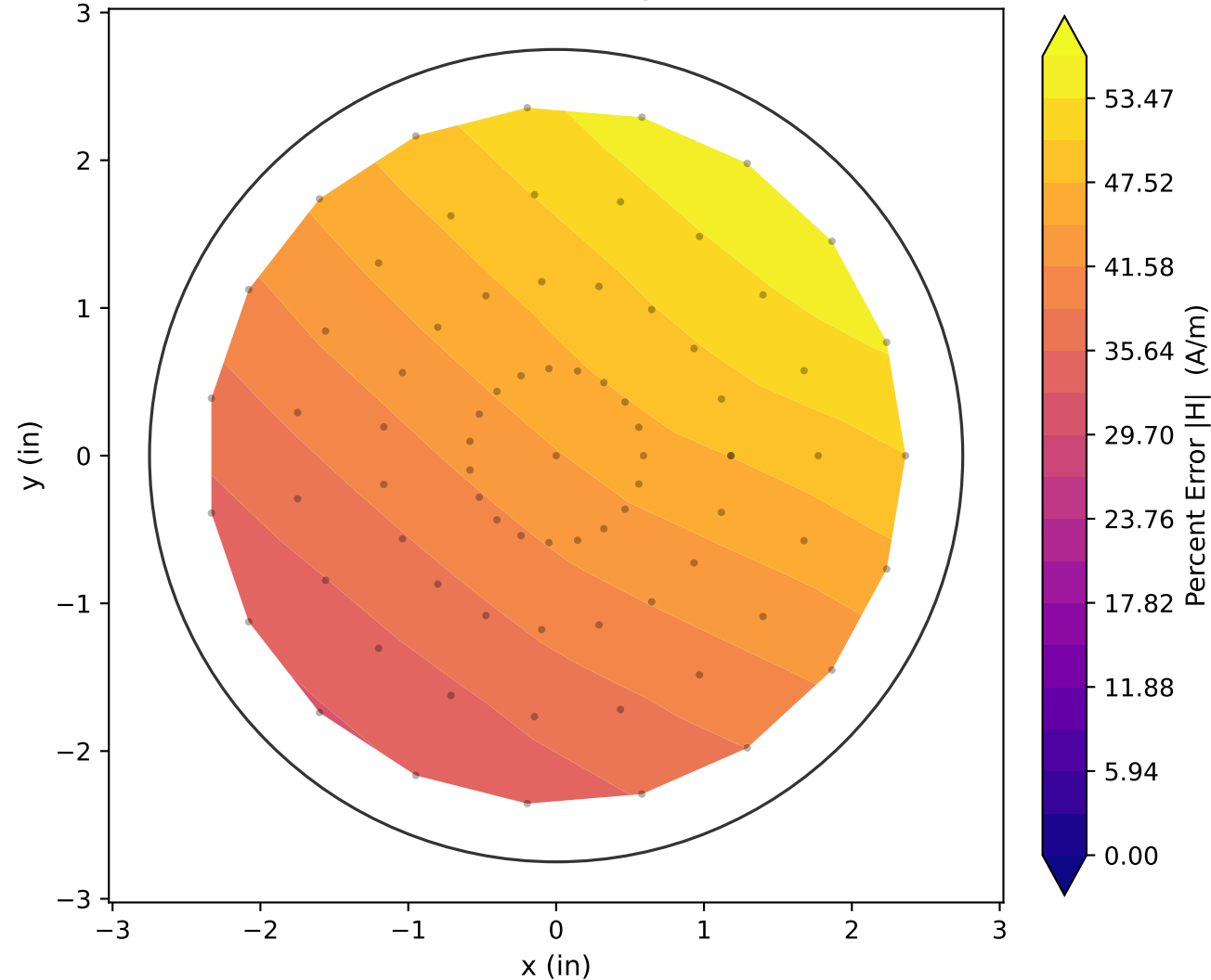
Reconstruction Error Percent — J=66.039 A/in 2 , slice 7
